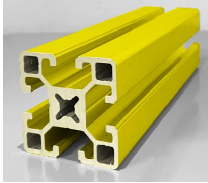
Frame Components
